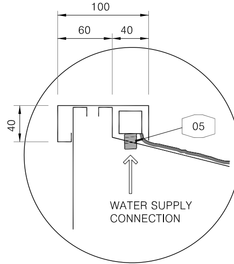
"A" PART DETAIL
