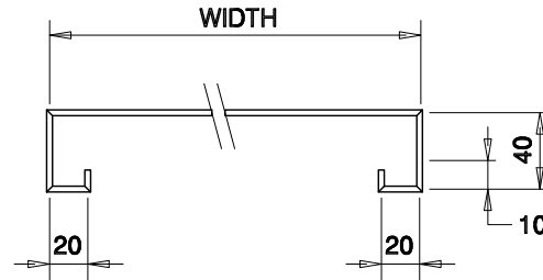
SECTION TOP
