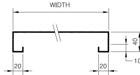
SECTION TOP
