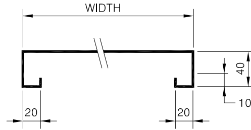
SECTION TOP
